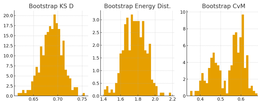
Figure 4: Bootstrap residual distribution from lattice spectra showing Wigner–Dyson spacing and GUE-type universality.
