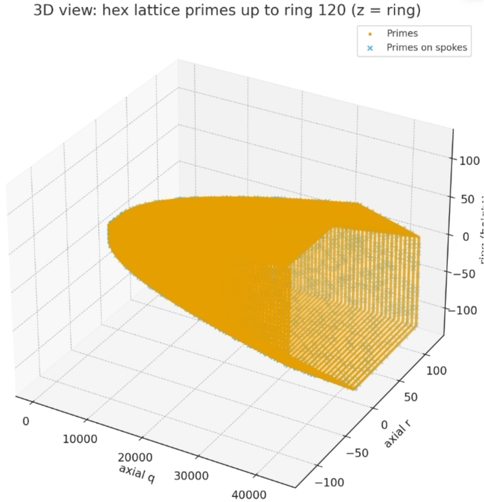
Figure 3: Allen Orbital Lattice operator: prime anchors (gold) and spoke-aligned primes (blue). The lattice defines the hexagonal indexing structure for the arithmetic operator described above.
